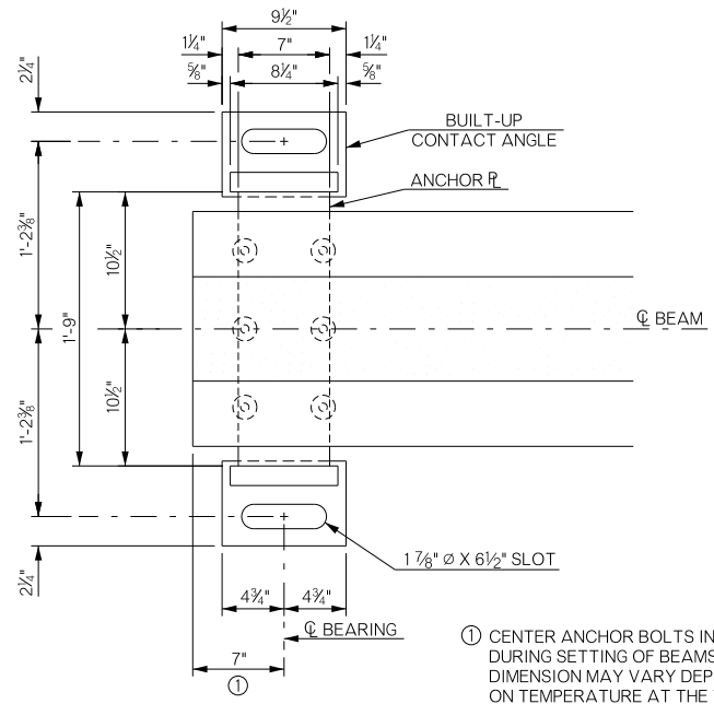
EXPANSION BEARING PLAN AT PIERS 1 & 2
