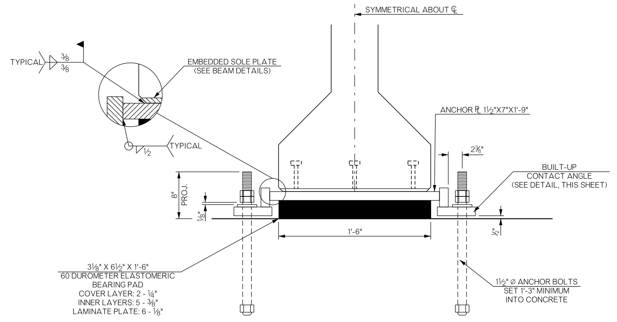
END VIEW
