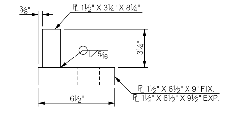
BUILT-UP CONTACT ANGLE DETAIL
