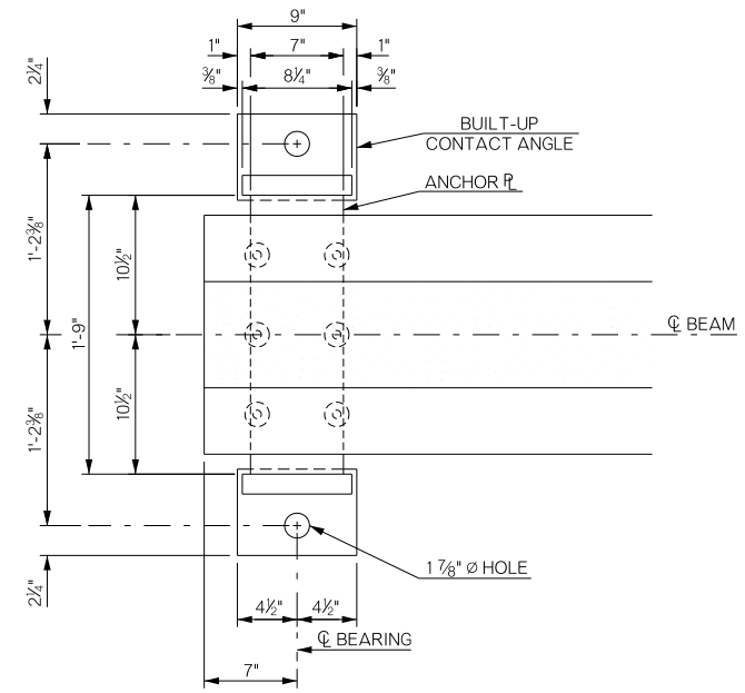
FIXED BEARING PLAN AT ABUTMENTS 1 & 2
